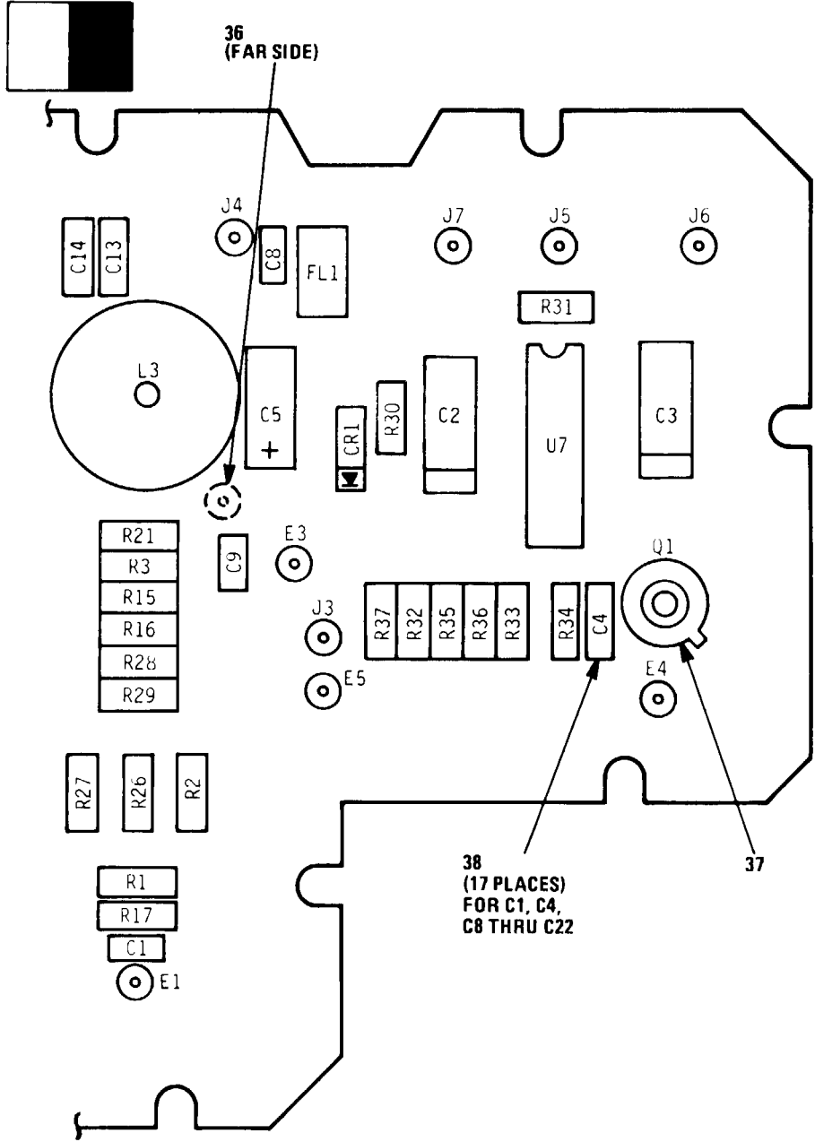
Figure 8. Oscillator Chain/Module Board No. 1 Circuit Card Assembly (3A3A1) (Sheet 2 of 2)
