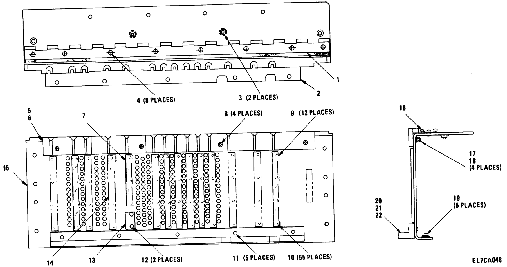
Figure 23. Left Panel Assembly (3A13)
