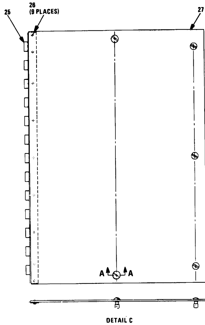
Figure 20. Chassis Subassembly (3A13) (Sheet 4 of 4)
