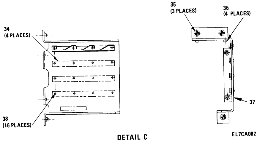
Figure 42. Chassis Assembly (4A7) (Sheet 4 of 5)
