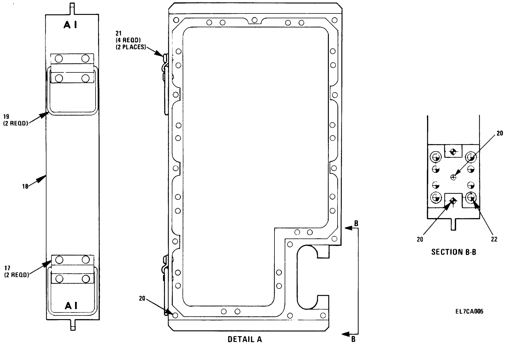
Figure 2. Mixer Preamp/VCO Buffer Module (3A1) (Sheet 3 of 3)
