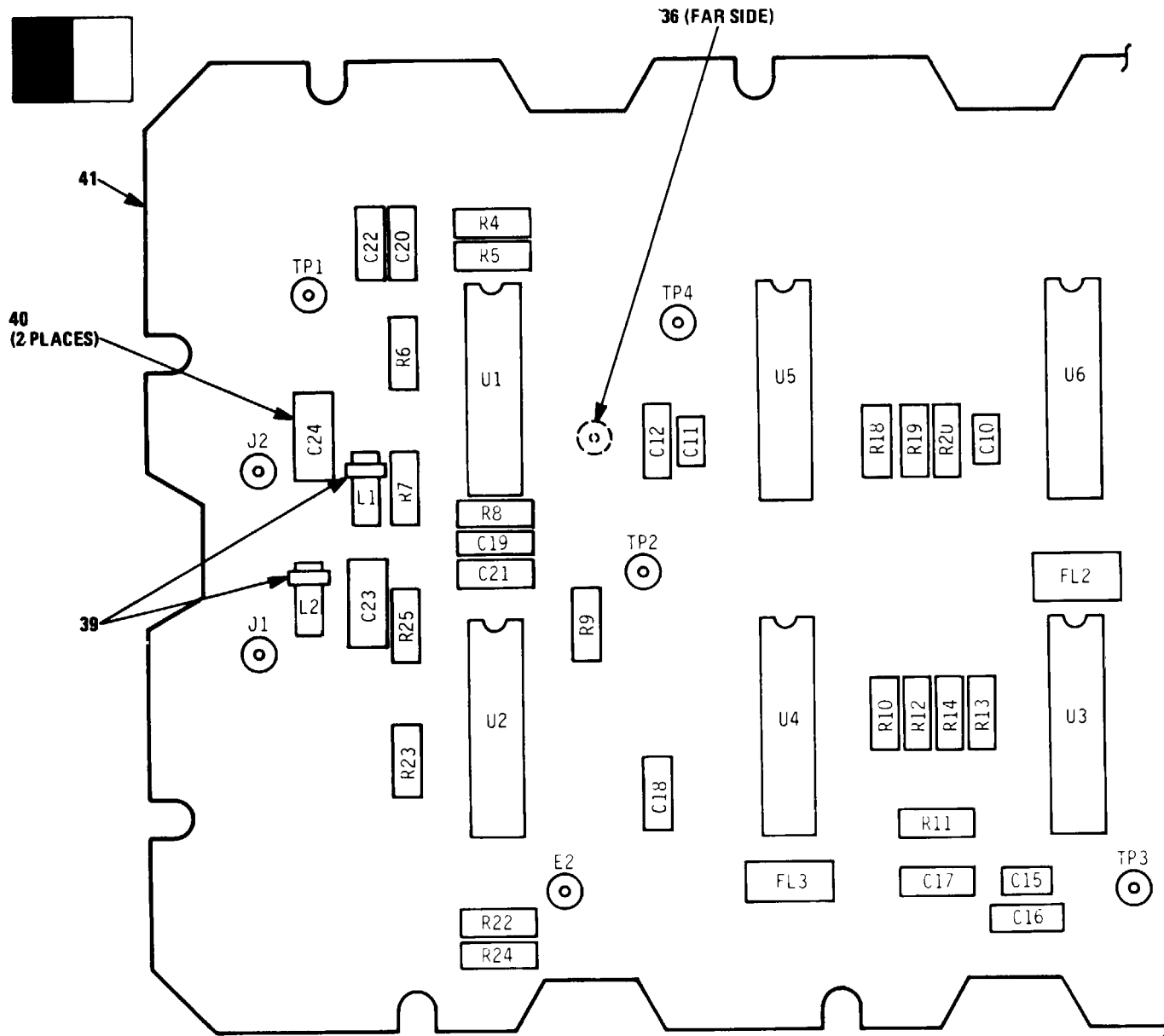
Figure 8. Oscillator Chain/Module Board No. 1 Circuit Card Assembly (3A3A1) (Sheet 1 of 2)
