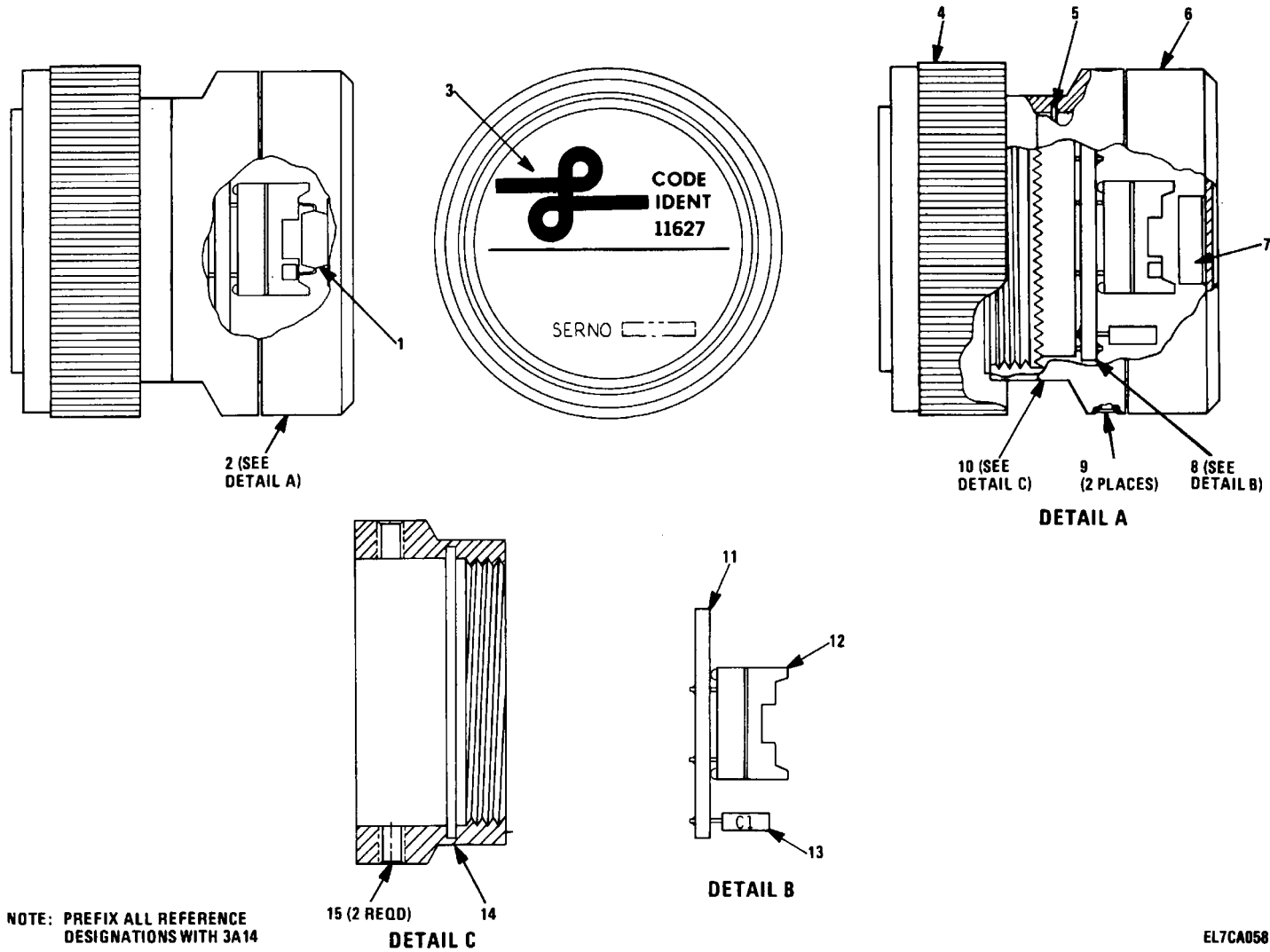
Figure 31. Memory Unit (3A14)
