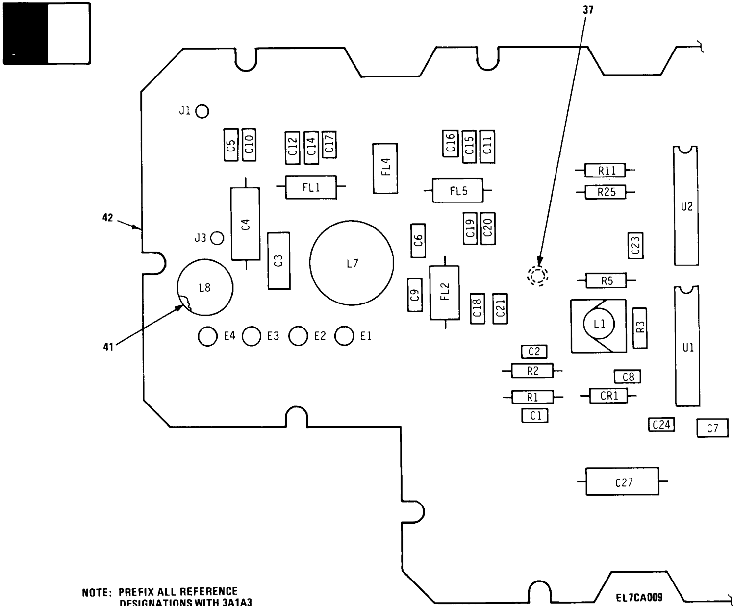
Figure 5. VCO Buffer Circuit Card Assembly (3A1A3) (Sheet 1 of 2)
