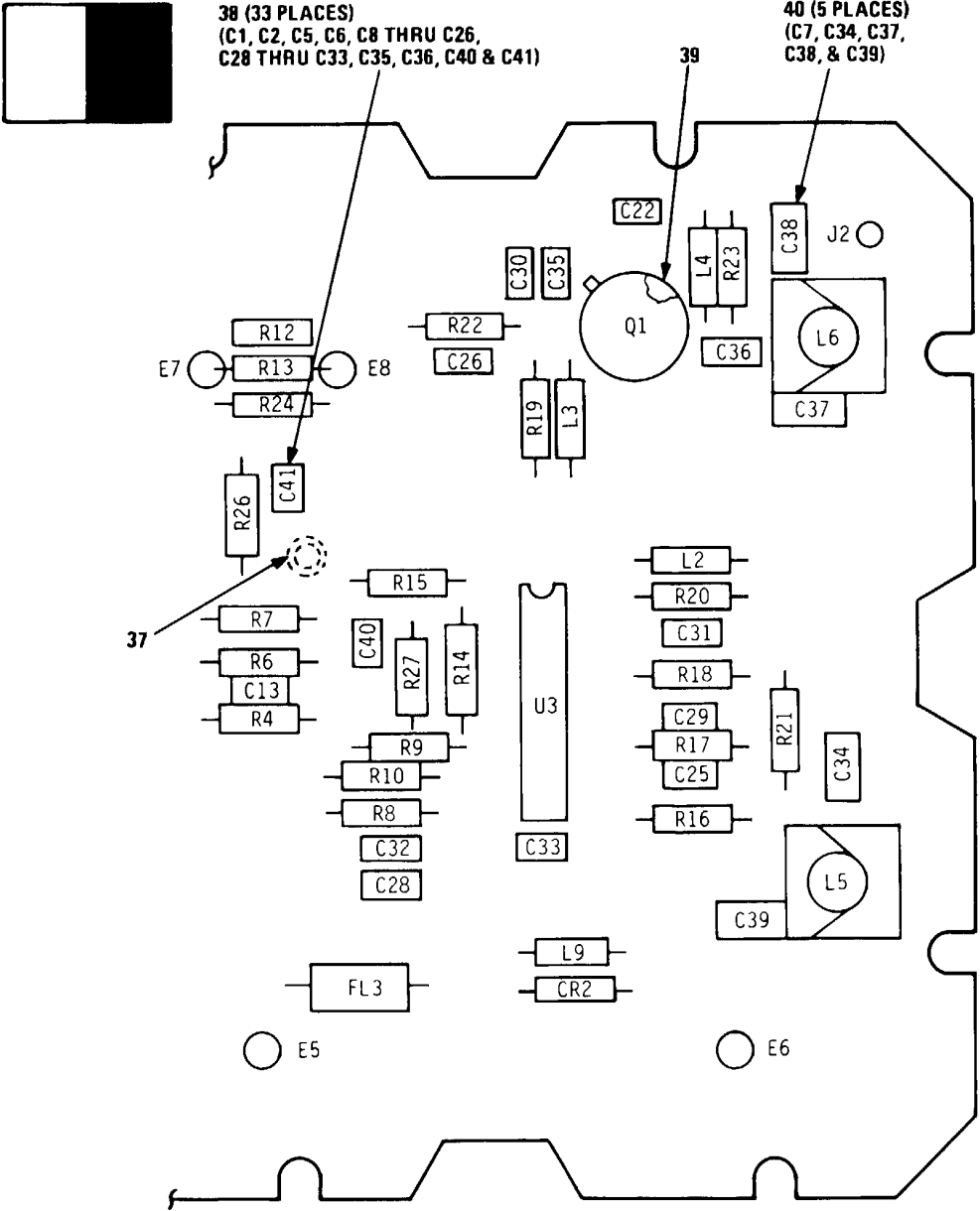
Figure 5. VCO Buffer Circuit Card Assembly (3A1A3), (Sheet 2 of 2)
