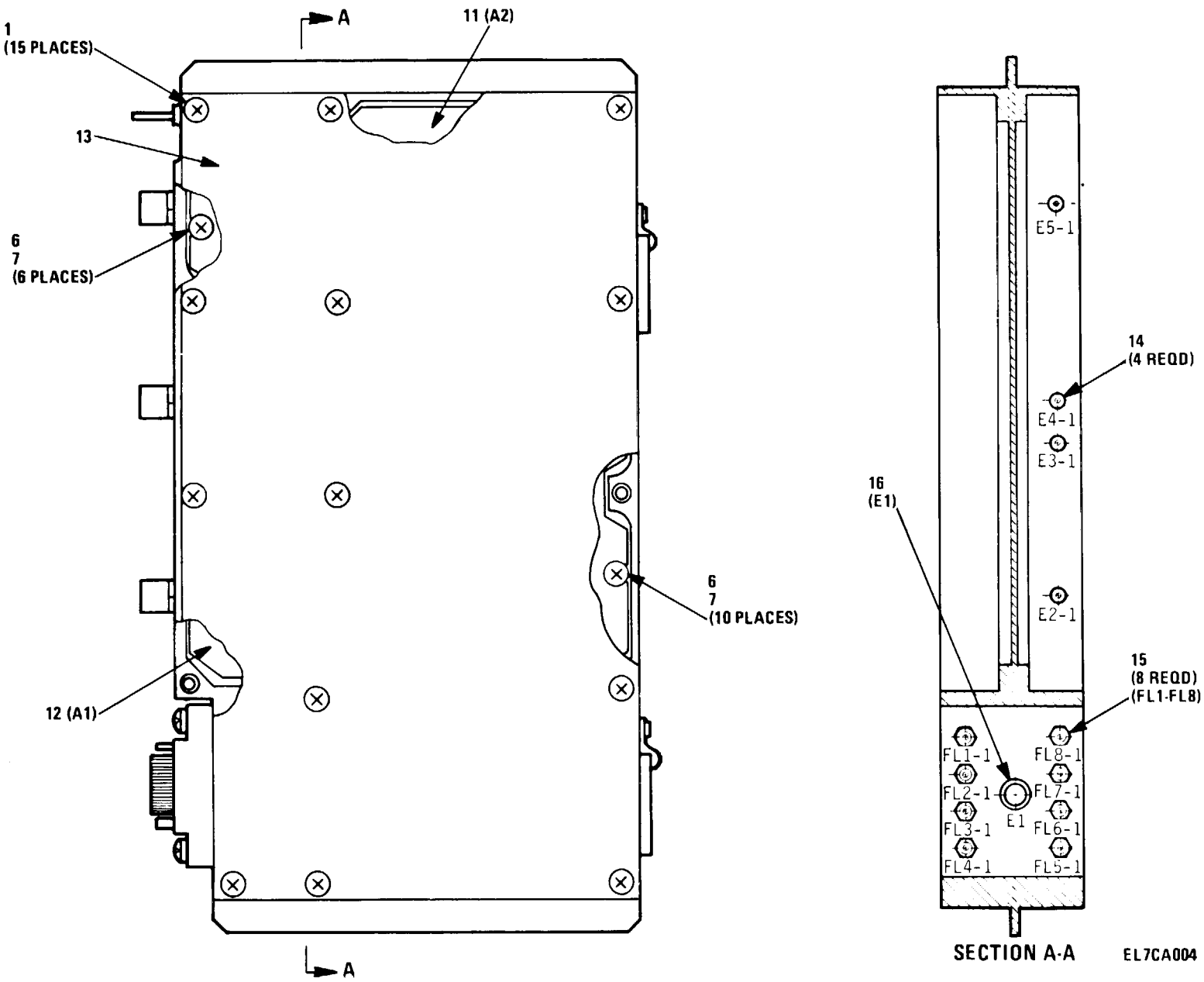
Figure 2. Mixer Preamp/VCO Buffer Module (3A1) (Sheet 2 of 3)
