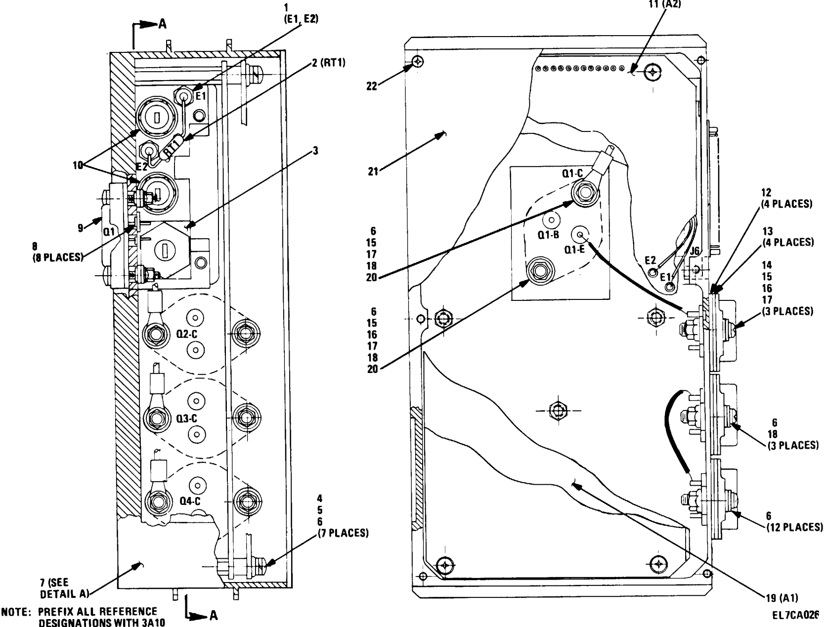
Figure 12. Power Supply Module (PA10) (Sheet 1 of 4)
