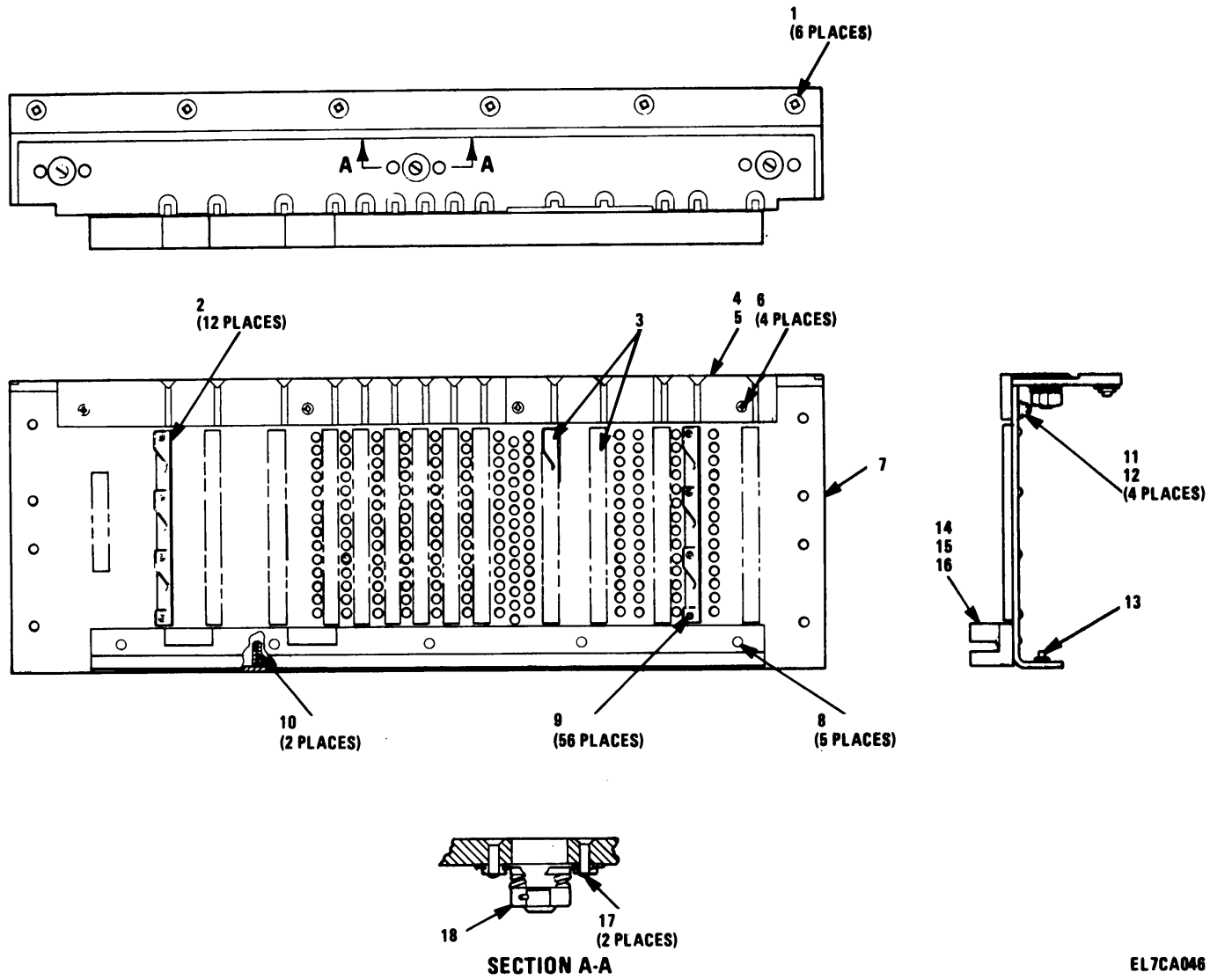
Figure 21. Right Panel Assembly (3A13)
