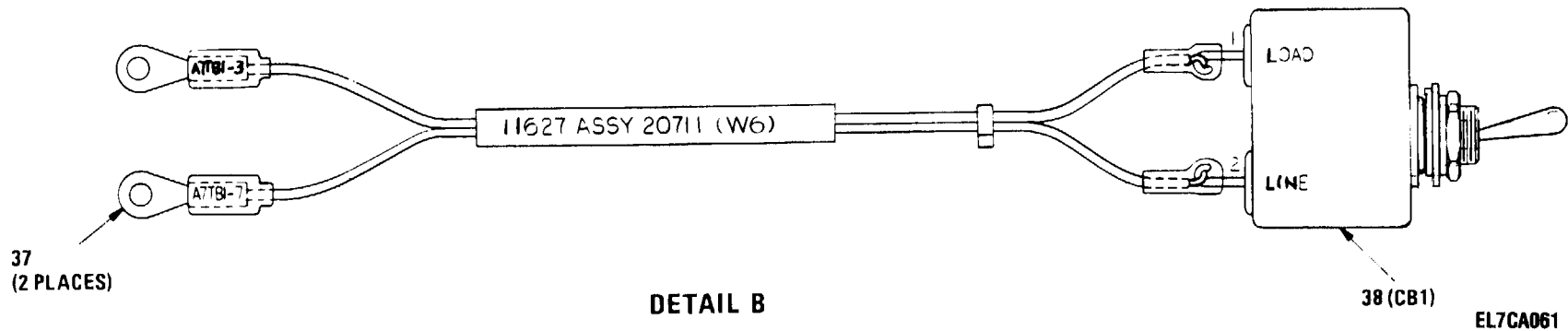
Figure 32. Control, Modem, Digital Data C-0812/G (4) (Sheet 3 of 3)
