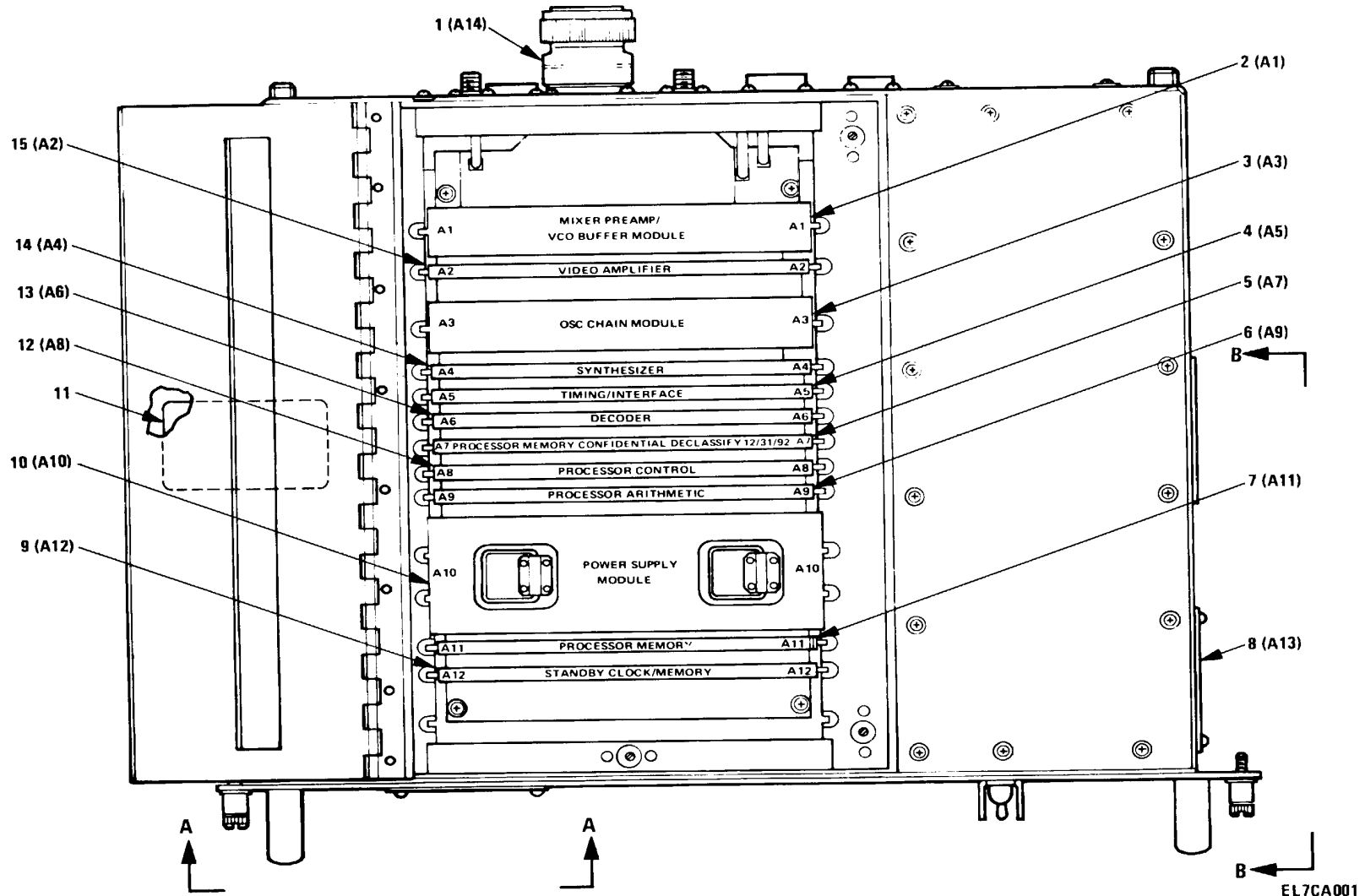
Figure 1. Modem, Digital Data MD-1094/G (3) (Sheet 1 of 2)
