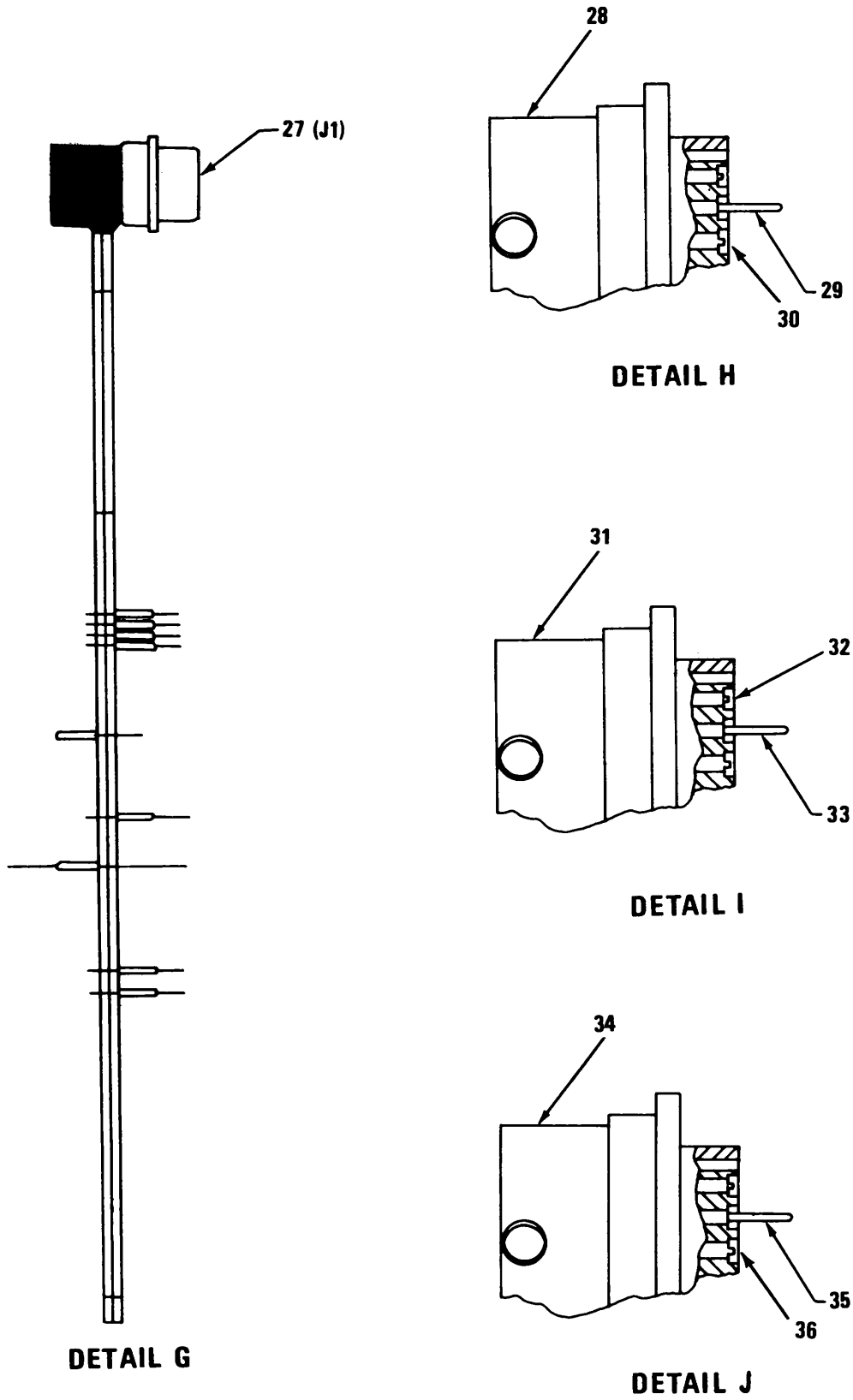
Figure 26. Rear Panel Assembly (3A13A1) (Sheet 3 of 3)
