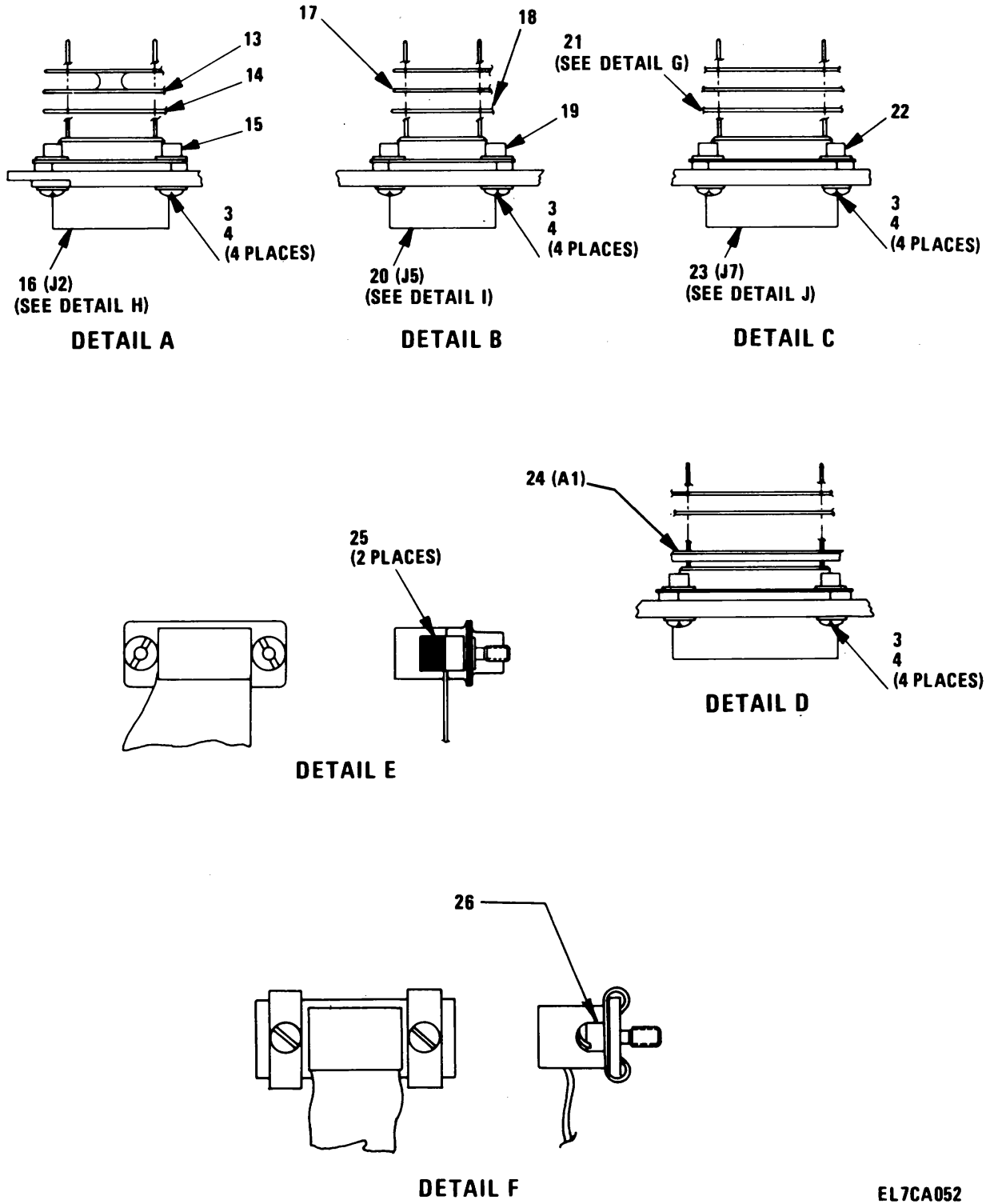
Figure 26. Rear Panel Assembly (3A13A1) (Sheet 2 of 3)
