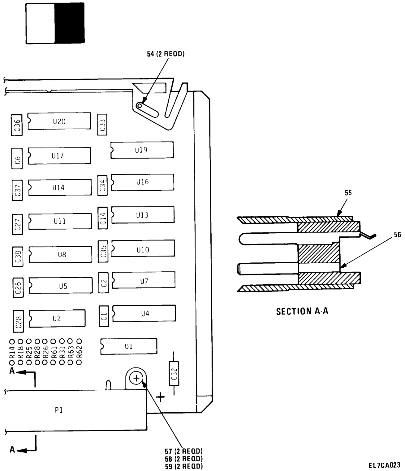
Figure 10. Timing Interface Circuit Card Assembly (3A5) (Sheet 2 of 3)
