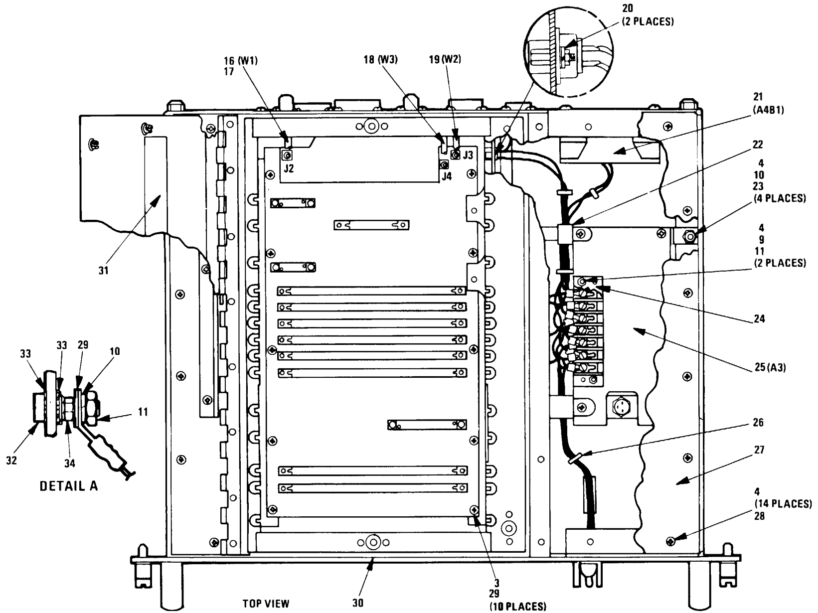
Figure 19. Chassis Assembly (3A13) (Sheet 2 of 2)
