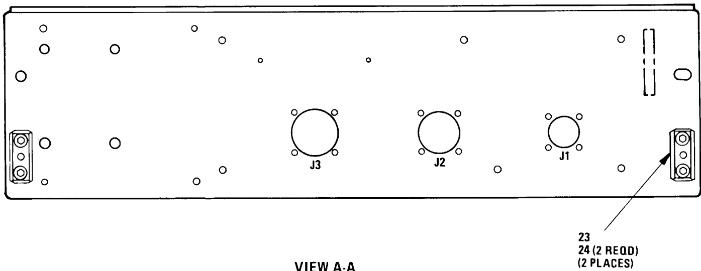
Figure 42. Chassis Assembly (4A7) (Sheet 2 of 5)
