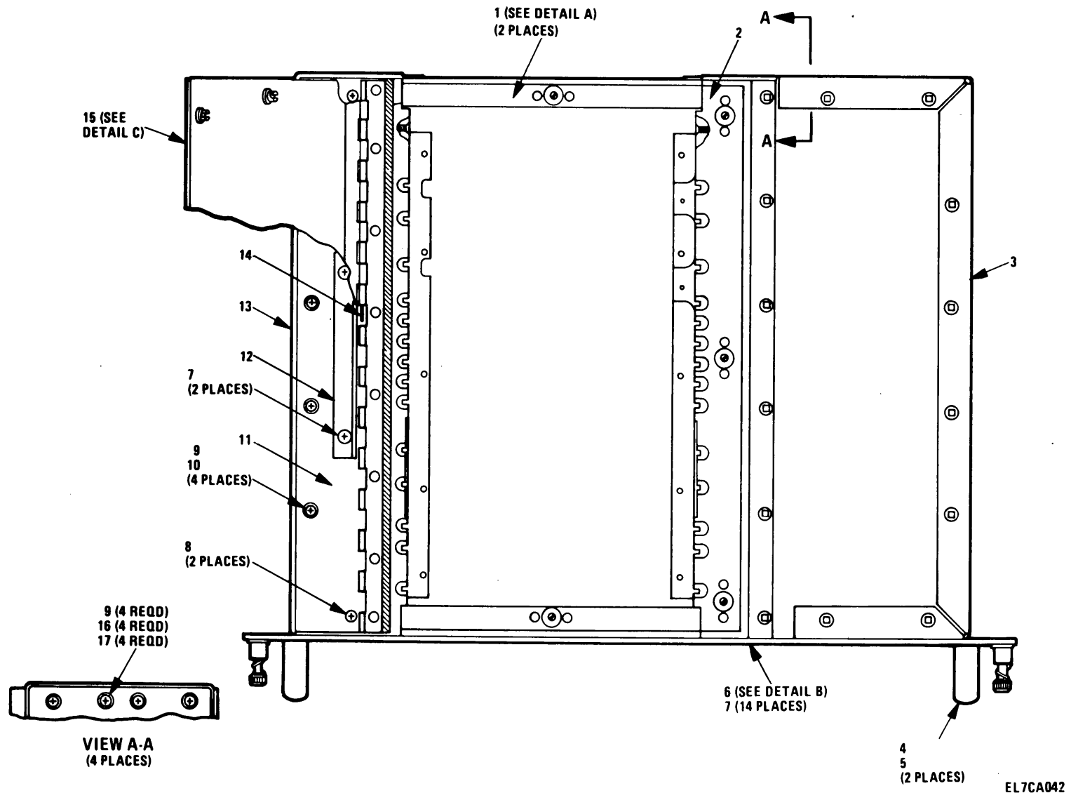
Figure 20. Chassis Subassembly (3A13) (Sheet 1 of 4)
