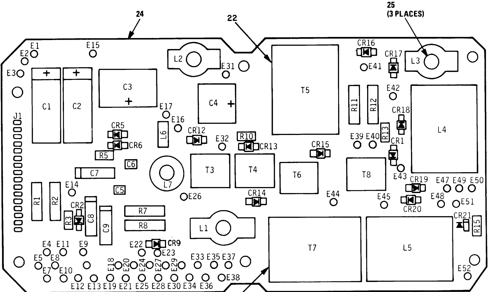
Figure 13. Power Supply Board No. 2 Circuit Card Assembly (3A10A1) (Sheet 1 of 2)
