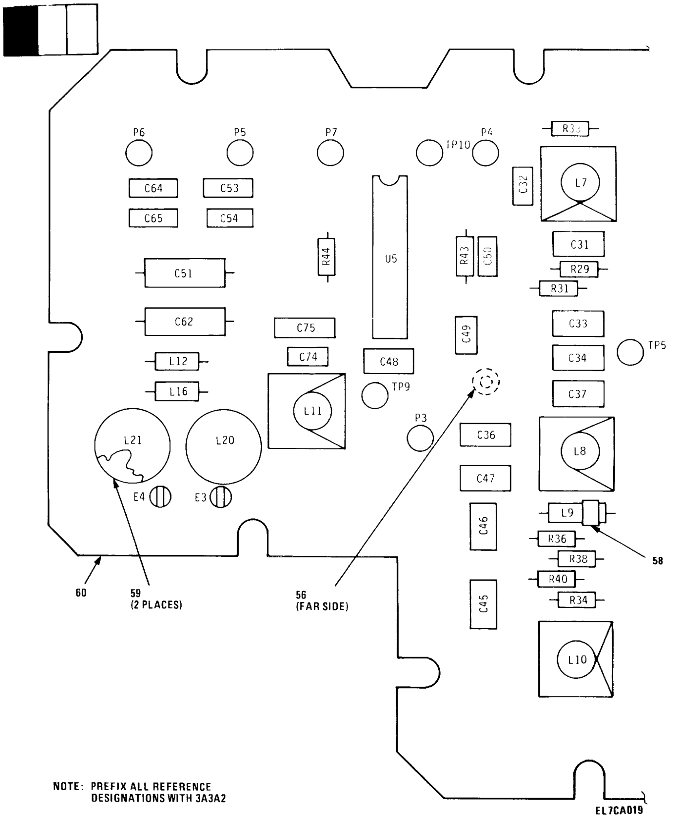
Figure 9. Oscillator Chain Module Board No. 2 Circuit Card Assembly (3A3A2) (Sheet 1 of 3)
