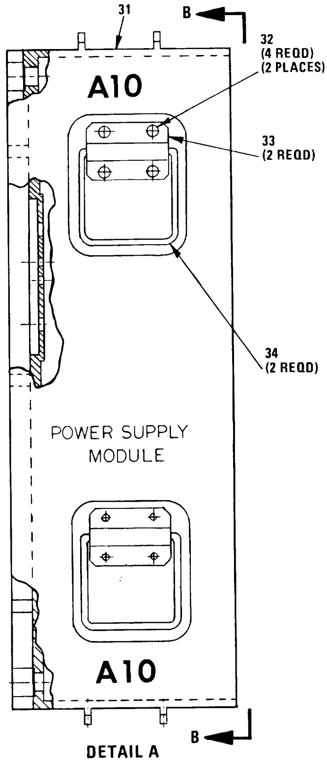
Figure 12. Power Supply Module (3A10) (Sheet 3 of 4)
