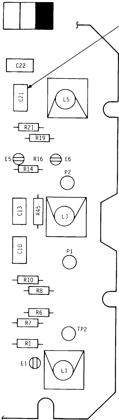
Figure 9. Oscillator Chain Module Board No. 2 Circuit Card Assembly (3A3A2) (Sheet 3 of 3)
