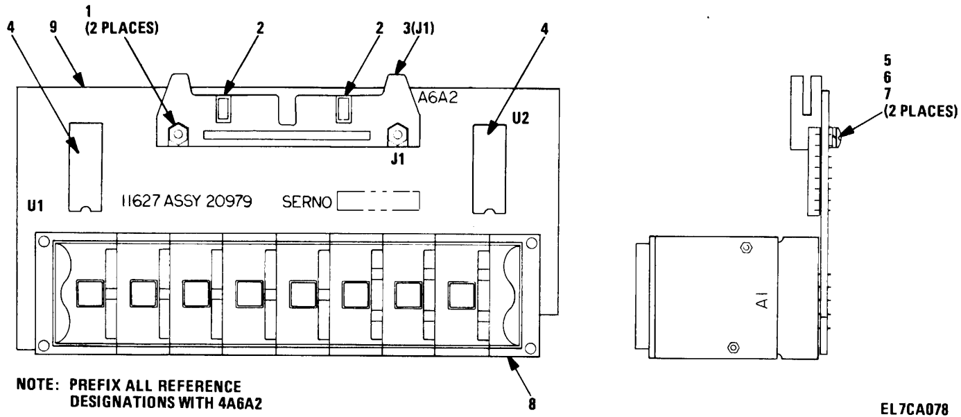
Figure 41. Front Panel Circuit Card Assembly (4A6A2)
