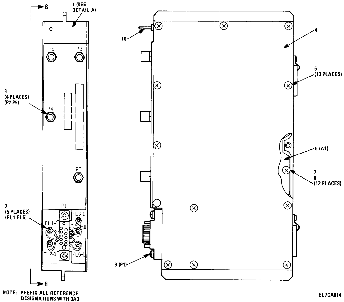
Figure 7. Oscillator Chain Module (3A3) (Sheet 1 of 3)
