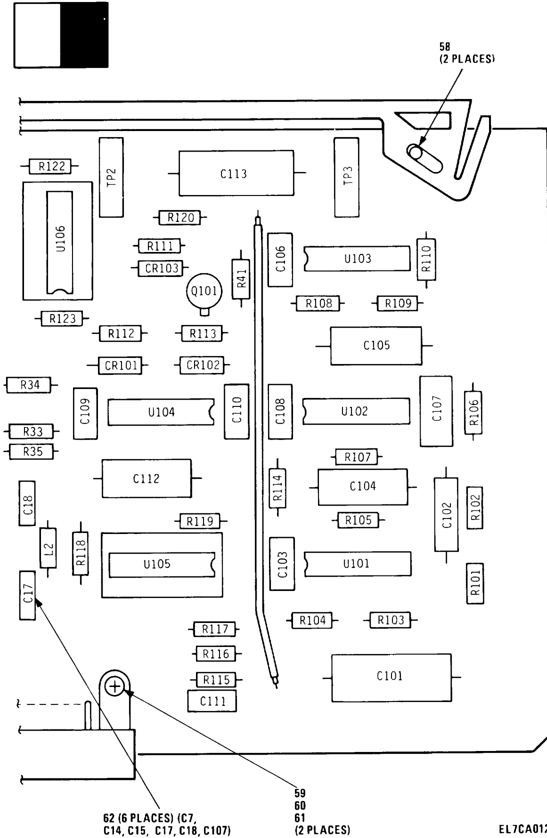
Figure 6. Video Amplifier Circuit Card Assembly (3A2) (Sheet 2 of 3)
