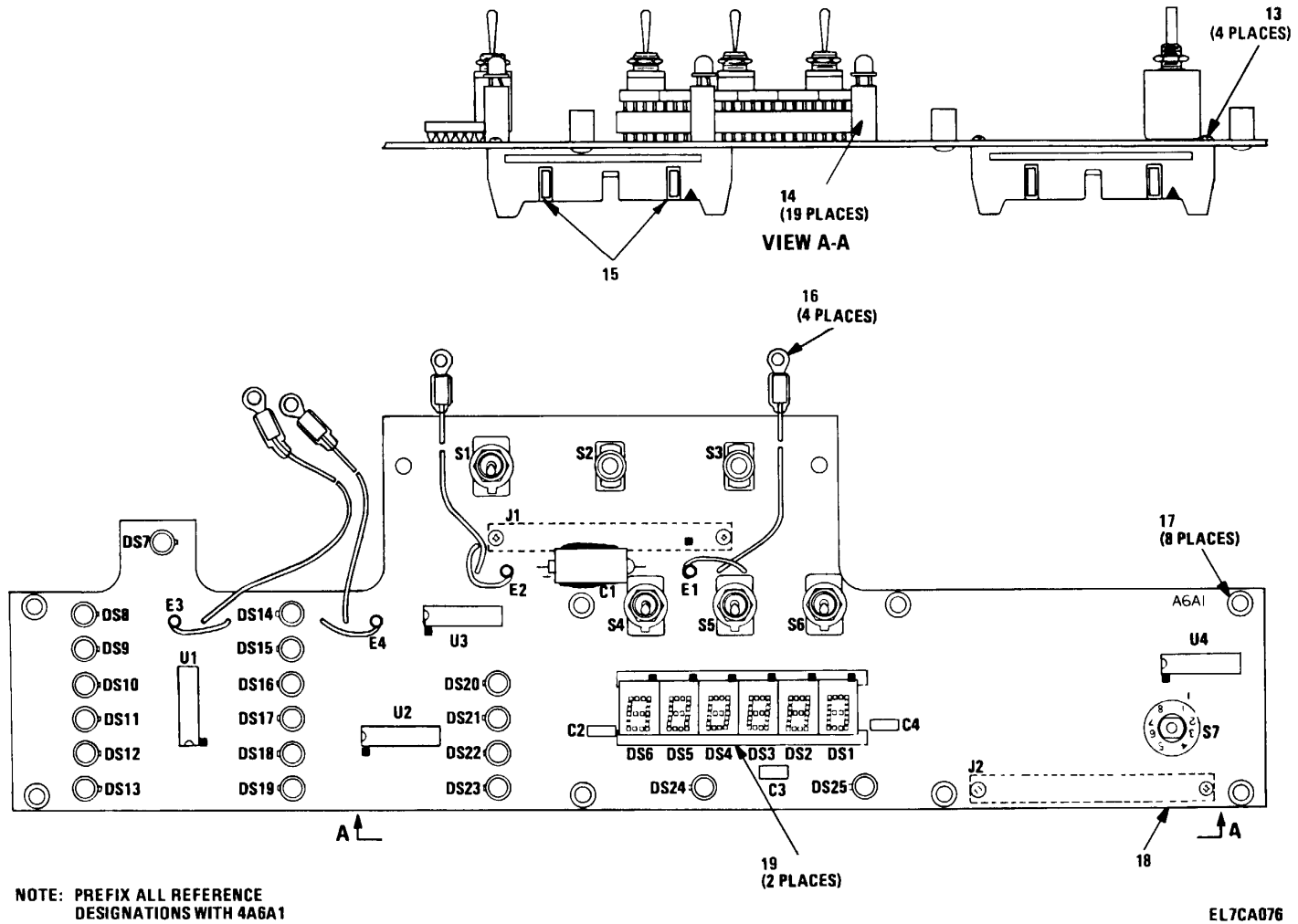
Figure 40. Switch Circuit Card Assembly (4A6A1) (Sheet 1 of 2)
