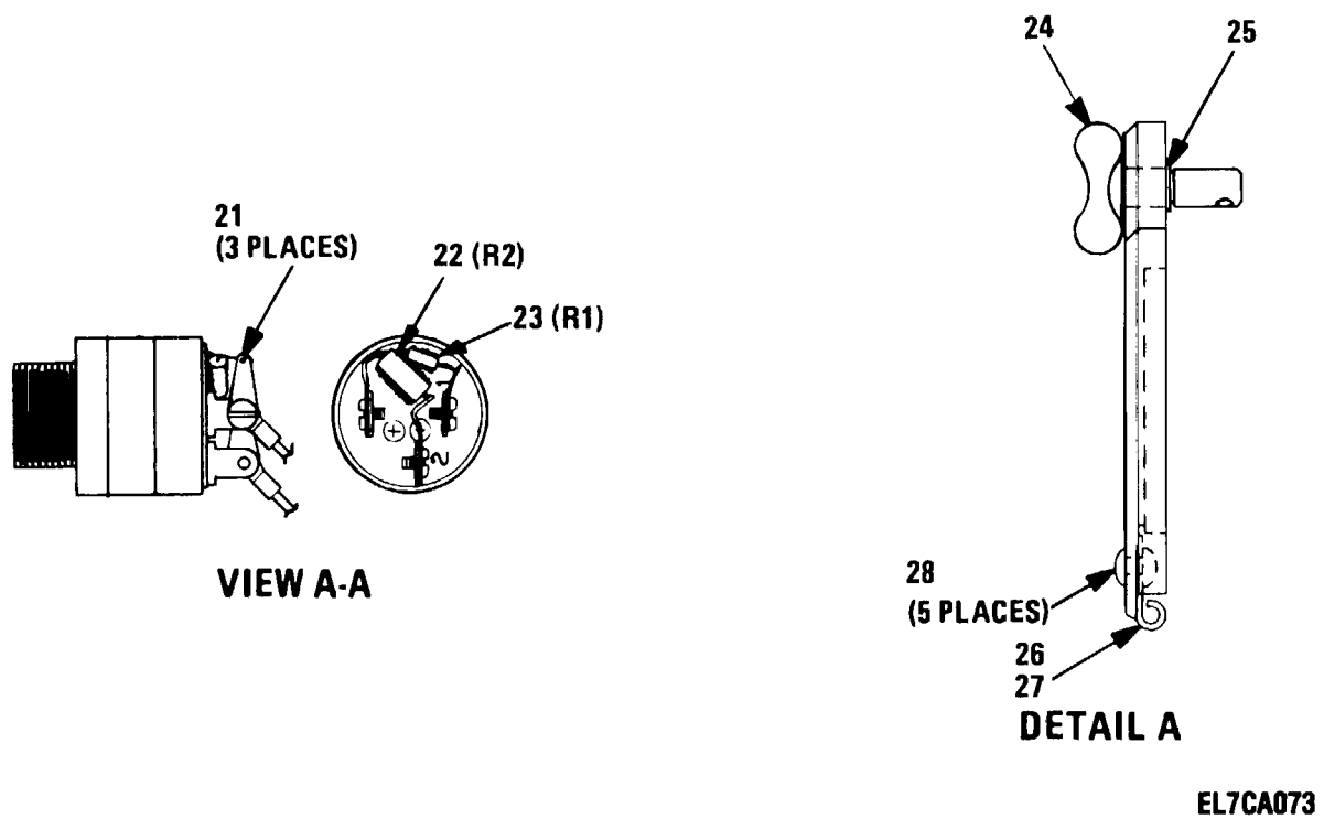
Figure 38. Front Panel Assembly (4A6) (Sheet 2 of 2)
