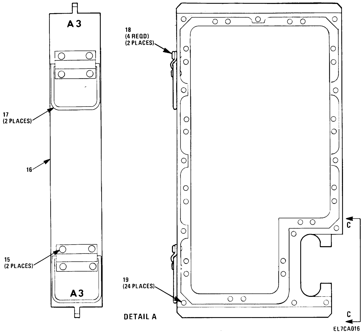
Figure 7. Oscillator Chain Module (3A3) (Sheet 3 of 3)
