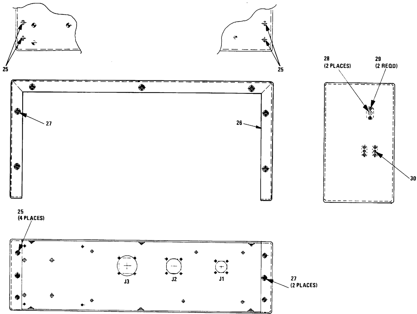
Figure 42. Chassis Assembly (4A7) (Sheet 3 of 5)
