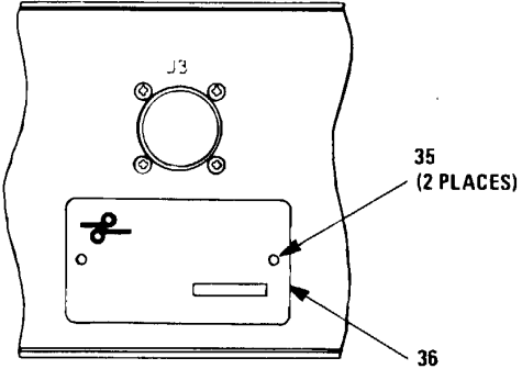
VIEW A-A ROTATED 180°
