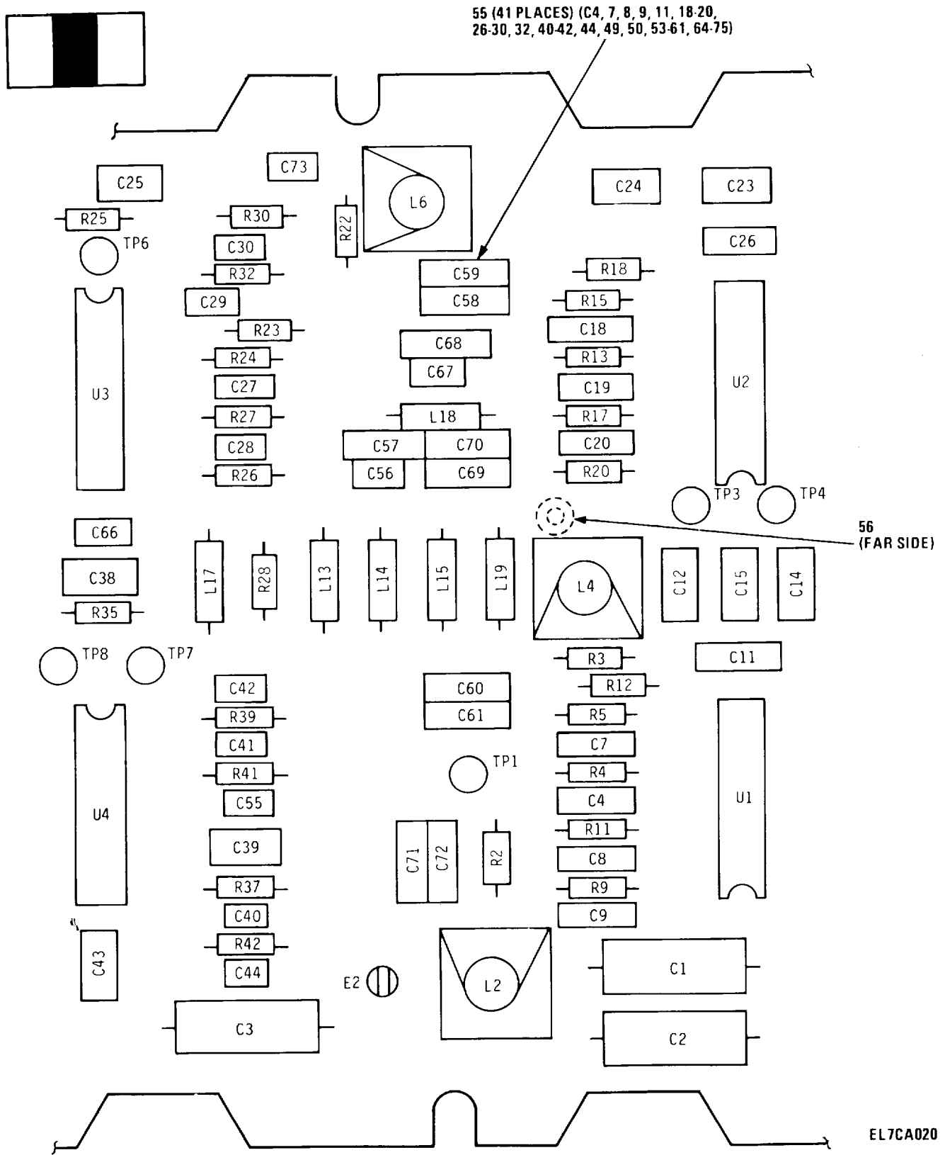
Figure 9. Oscillator Chain Module Board No. 2 Circuit Card Assembly (3A3A2) (Sheet 2 of 3)
