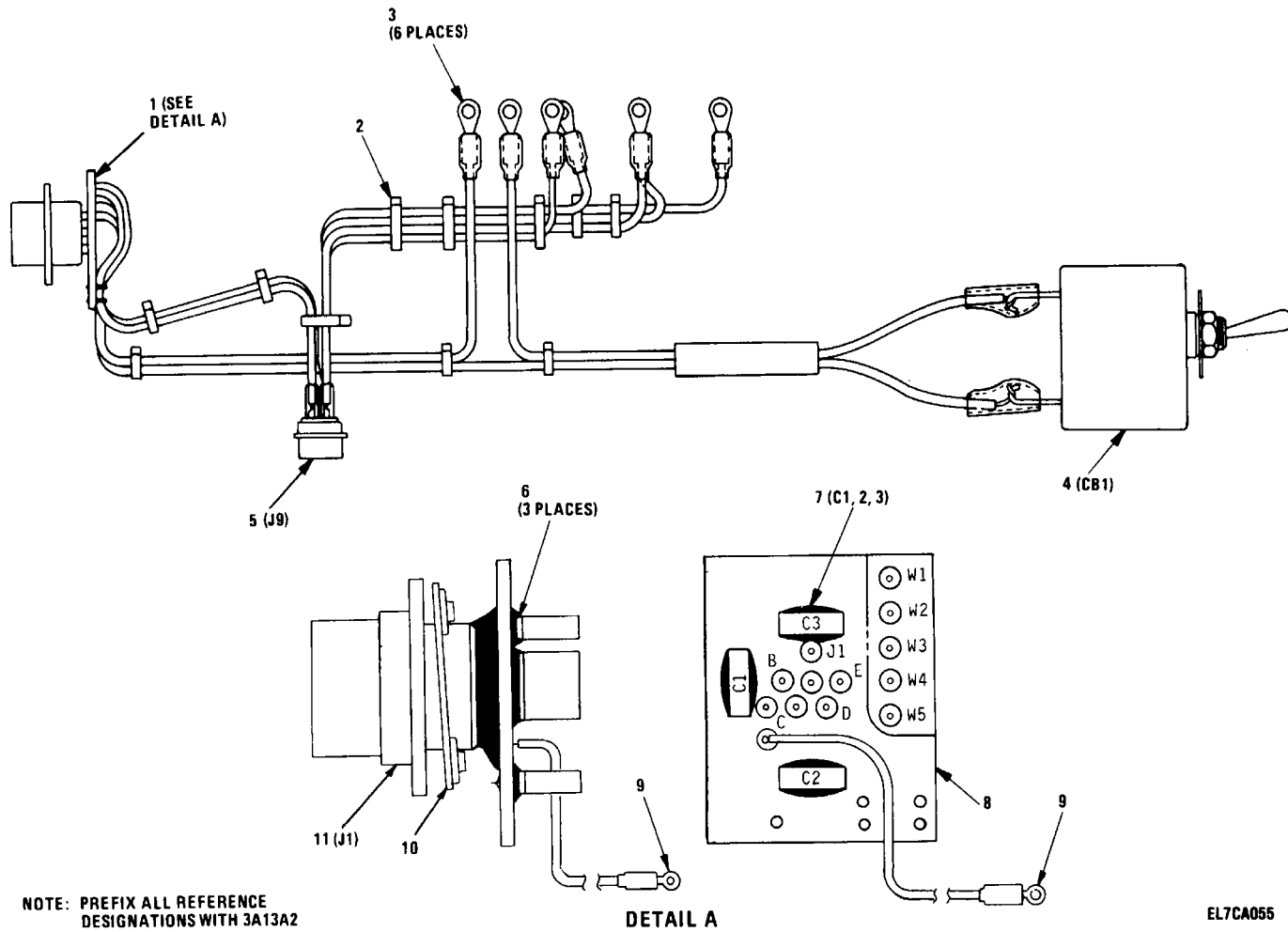
Figure 28. Power Harness (3A13A2)
