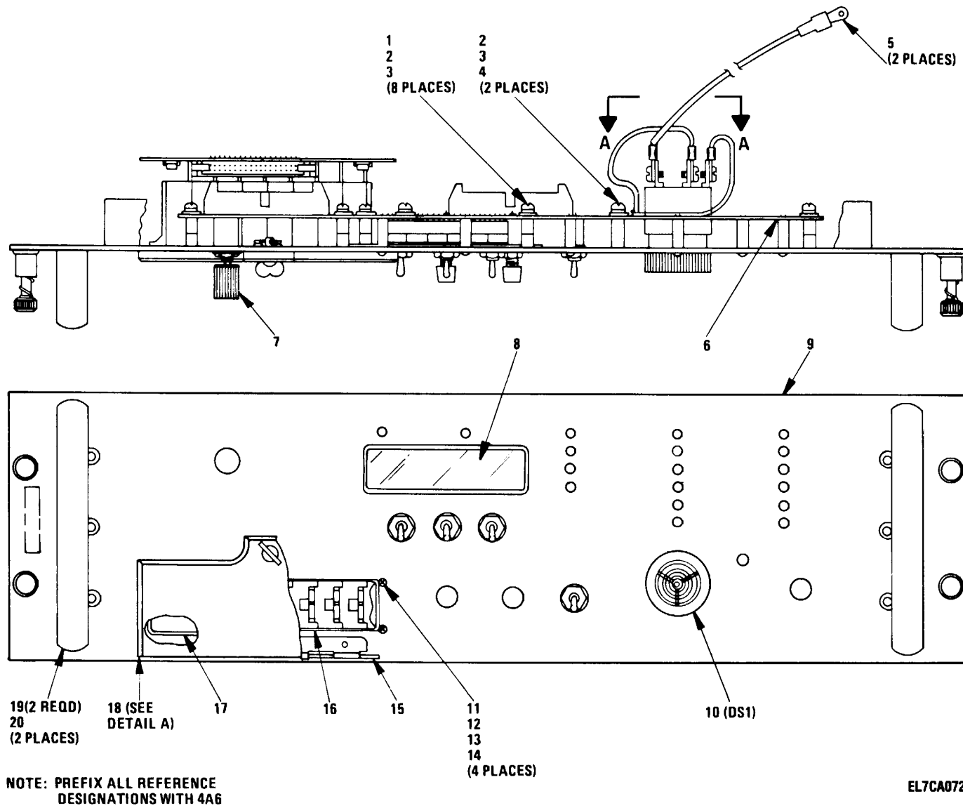
Figure 38. Panel Assembly (4A6) (Sheet 1 of 2)
