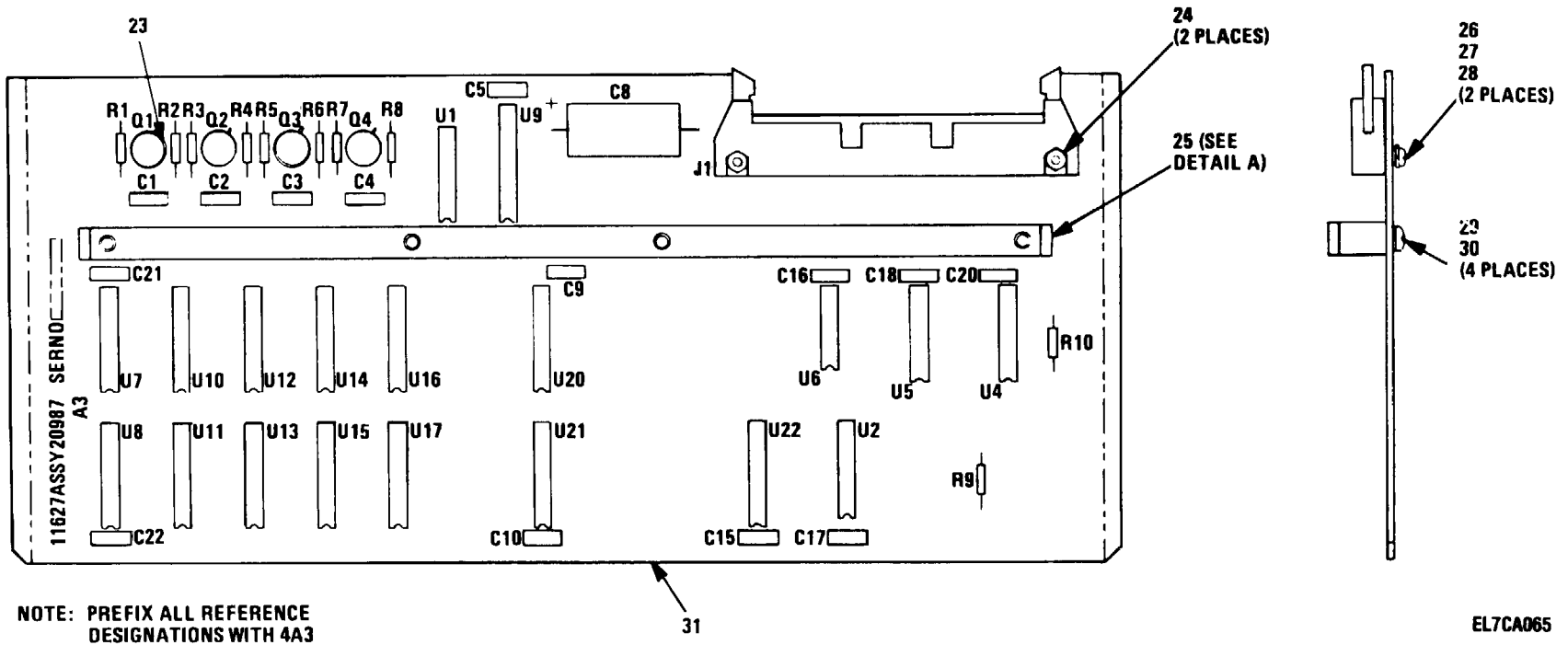
Figure 35. Memory Circuit Card Assembly (4A3) (Sheet 1 of 2)
