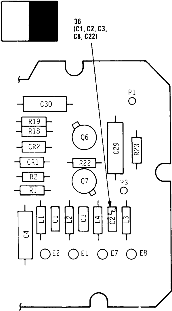
Figure 4. Mixer Preamp Board No. 2 Circuit Card Assembly (3A1A2) (Sheet 2 of 2)
