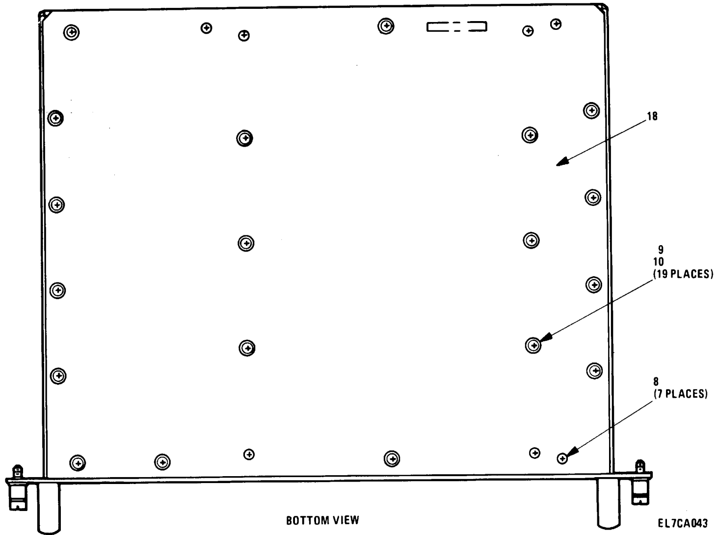
Figure 20. Chassis Subassembly (3A13) (Sheet 2 of 4)
