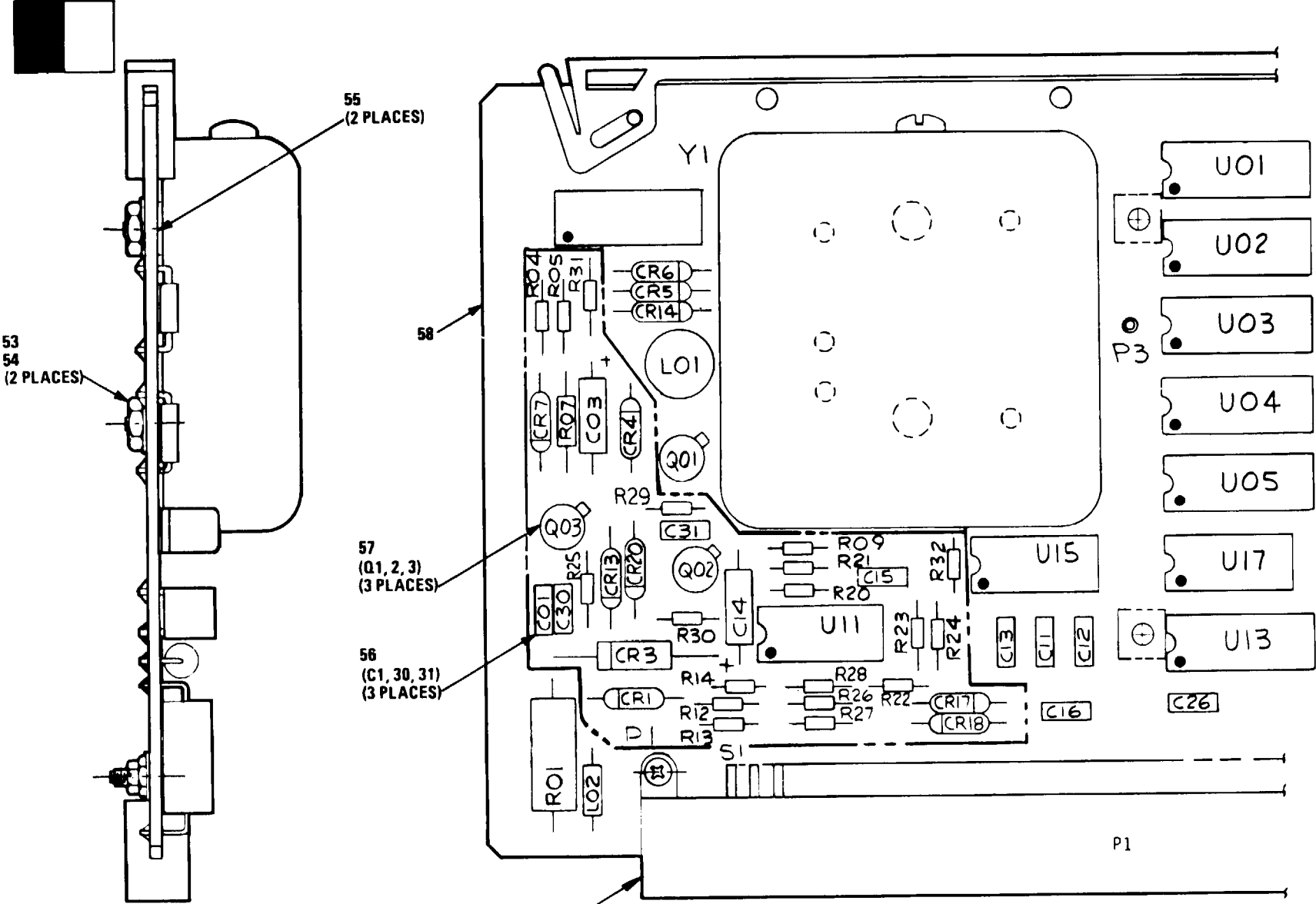
Figure 17. Standby Clock Memory Circuit Card Assembly (3A12A2) (Sheet 1 of 2)
