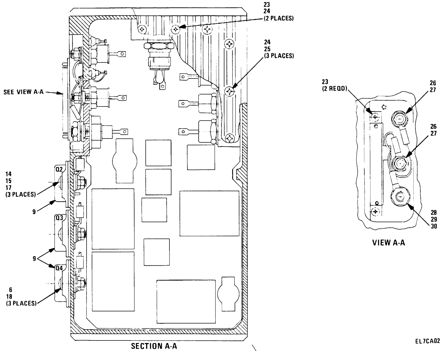
Figure 12.. Power Supply Module (3A10) (Sheet 2 of 4)
