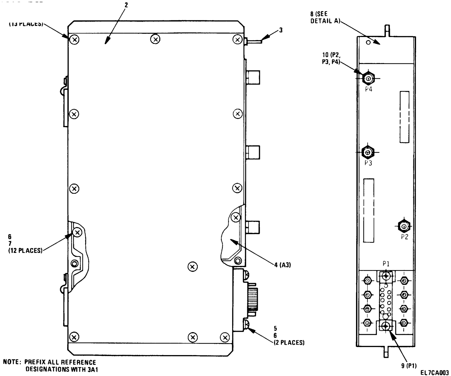
Figure 2. Mixer Preamp/VCO Buffer Module (3A1) (Sheet 1 of 3)
